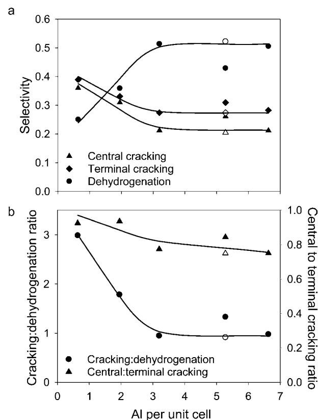
Figure 5. Selectivities (a) and selectivity ratios (b) for monomolecular n -butane reactions versus Al atoms per unit cell in H-MFI. Data for MFI-15(M), which was treated with EDTA, are indicated with hollow symbols.
