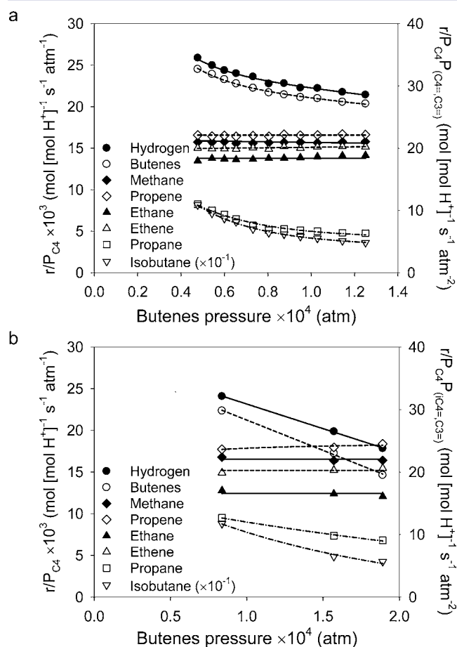
Figure 9. (a) Rates of monomolecular reactions (left axis) and secondary hydride transfer reactions (right axis) versus butene partial pressure for MFI-11.5 at 773 K and a space time of 0.09 [s (mol \text{H}^+ ) (mol feed) -1 ]. Conversion is constant at 0.57 \pm 0.02 %. (b) Rates of reactions as stated in (a), but with varying levels of isobutene introduced as co-feed. Horizontal axis indicates the total partial pressure of butenes.
